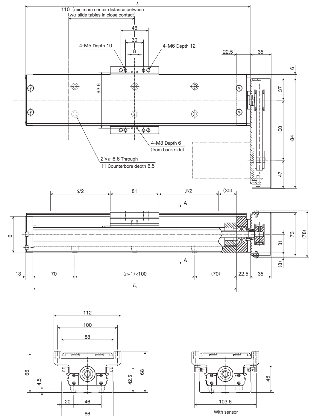
A-A Sectional dimension unit: mm
